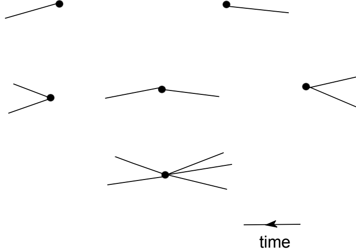
Figure 1: Various Friedrichs vertices
