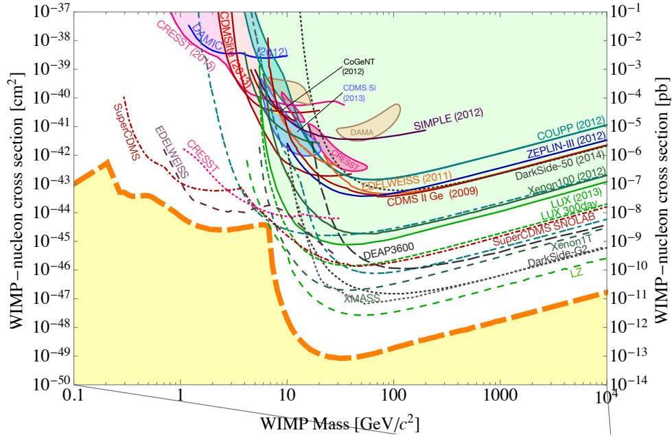
Figure 1: Limits or evidence (as claimed by the authors) for the cross section for DM-nucleon interactions, source P. Cushman et al., arXiv:1310.8327
