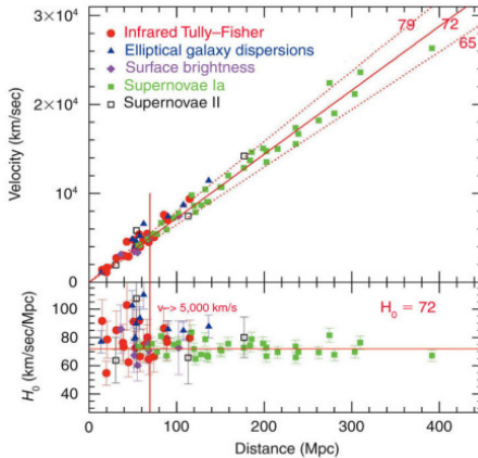
Figure 3: The Hubble diagram for the redshift interpreted as a non-relativistic Doppler effect. The Hubble's law works very well up to distances of many hundred Mpc.
